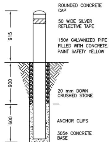
BOLLARD DETAIL
